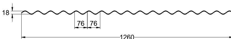
PROFILE: Oo2/18-76/1260
